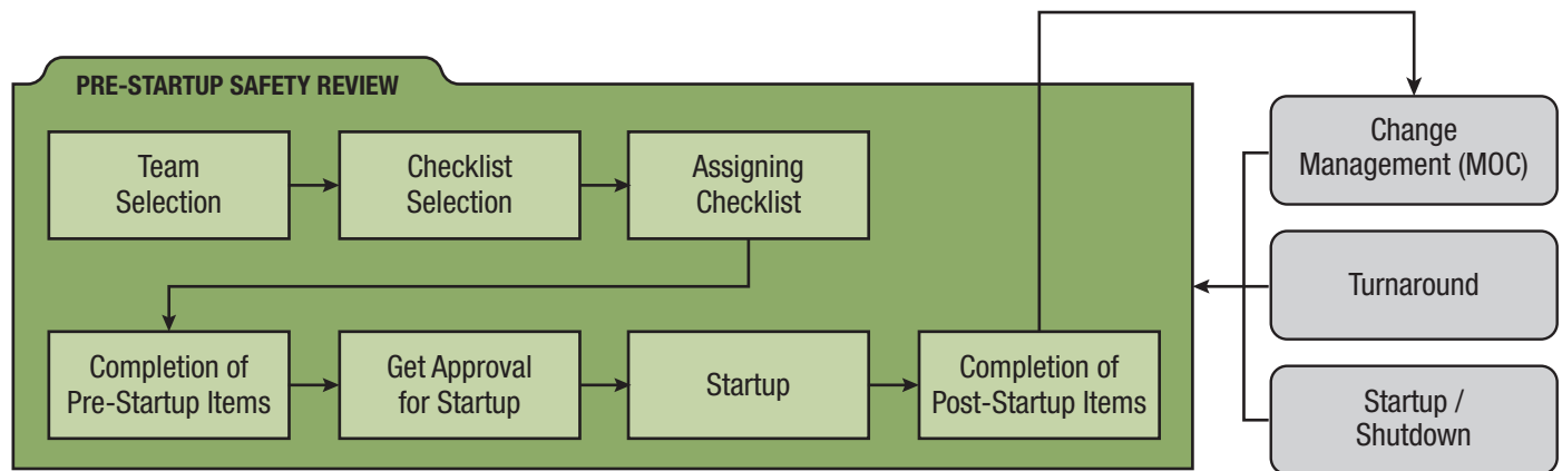
Figure 1 – PSSR Process in OESuite
